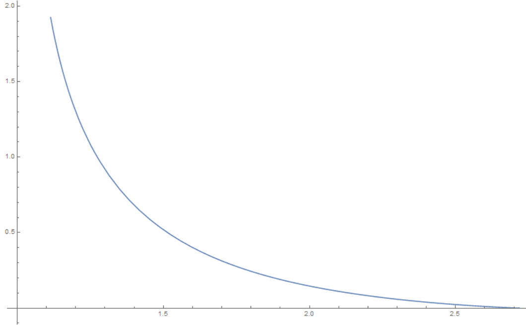
Figure 3: Innate cost density based on estimate of Gagnepain and Ivaldi (2002, Table 3)
