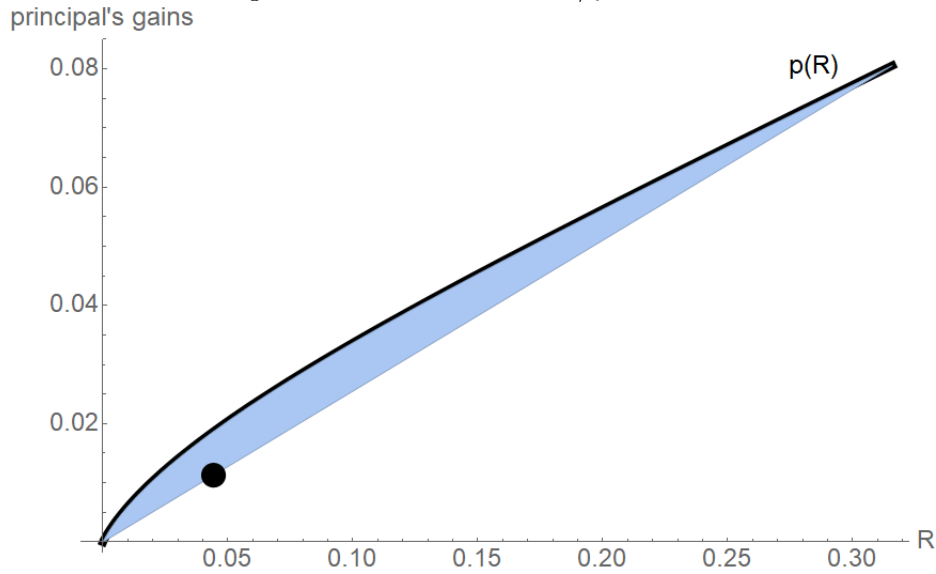
Figure 2: Example with F/f concave
