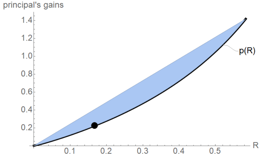
Figure 1: Example with F/f convex
