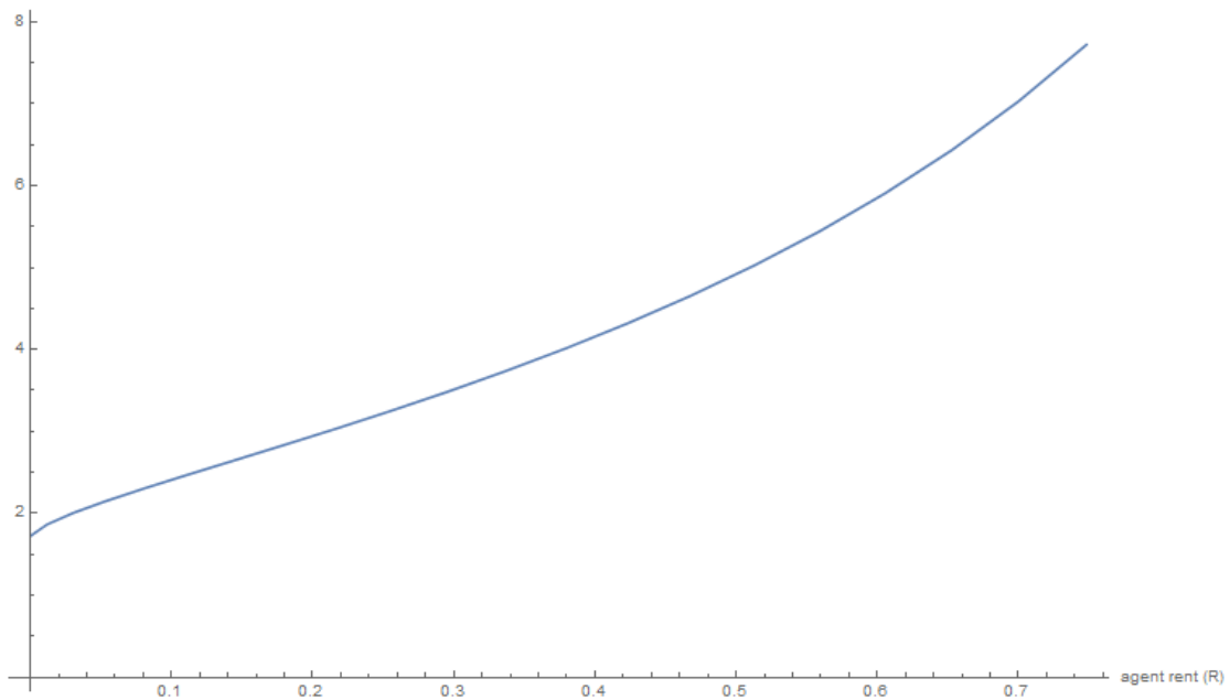
Figure 4: Ratio of gains to rents ( G^{\text{inf}}(R)/R ) against agent rents ( R ) for density of Figure 3
